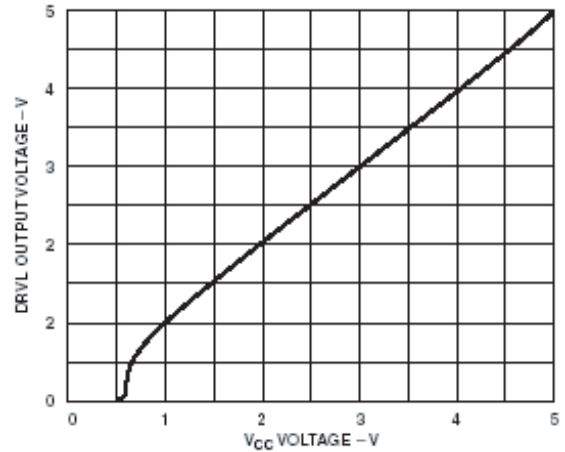
DRVL Output Voltage vs. Supply Voltage
