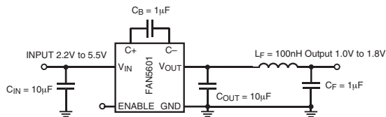
Figure 2. Optional L-C Filter
