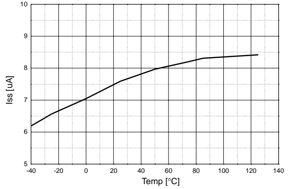
Figure 8. Soft Start Current
