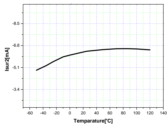
Figure 11. Output Source Current 2
