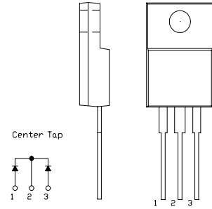
OUTLINE DRAWING
