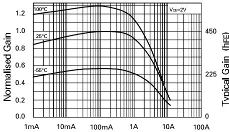
Collector Current
