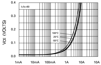
Collector Current
