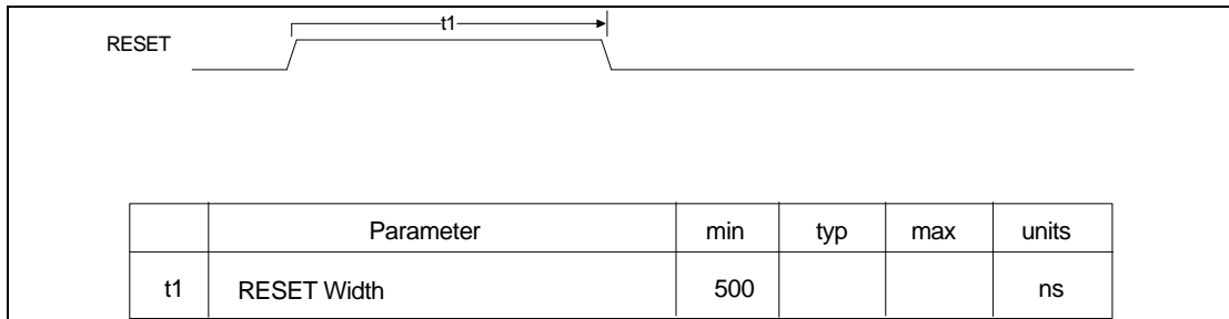
FIGURE 7 - RESET TIMING
