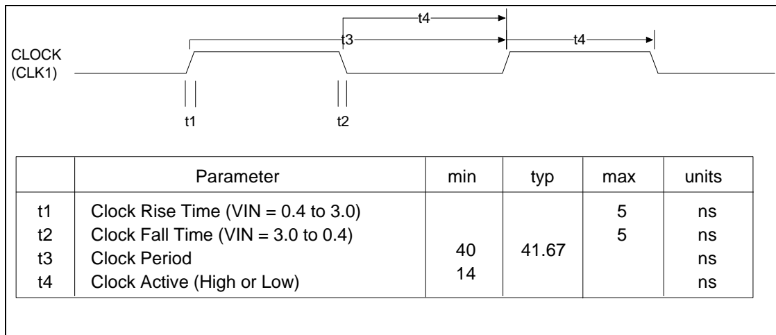
FIGURE 8 - CLOCK TIMING
