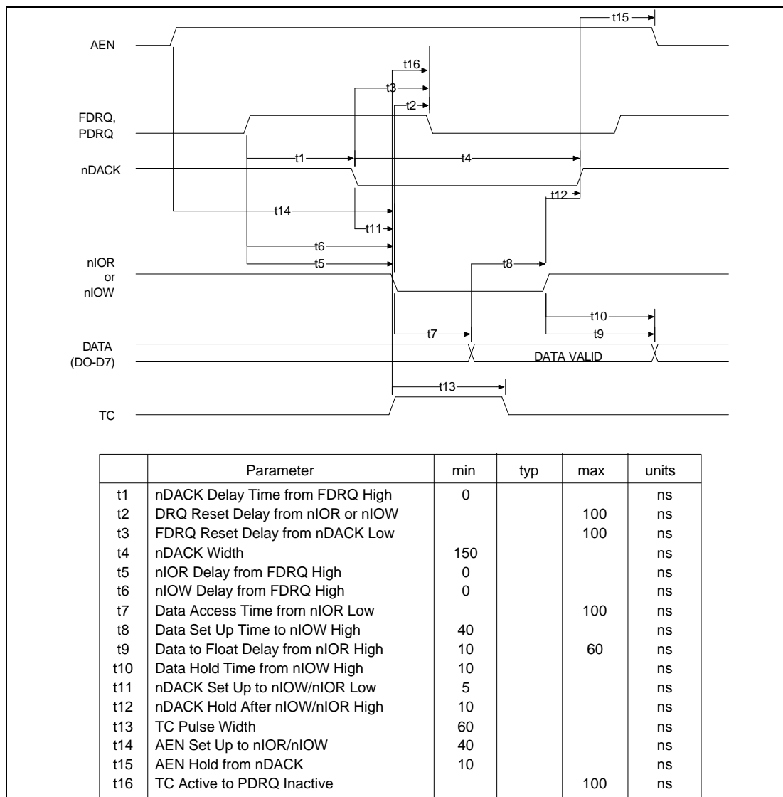
FIGURE 6 - DMA TIMING
