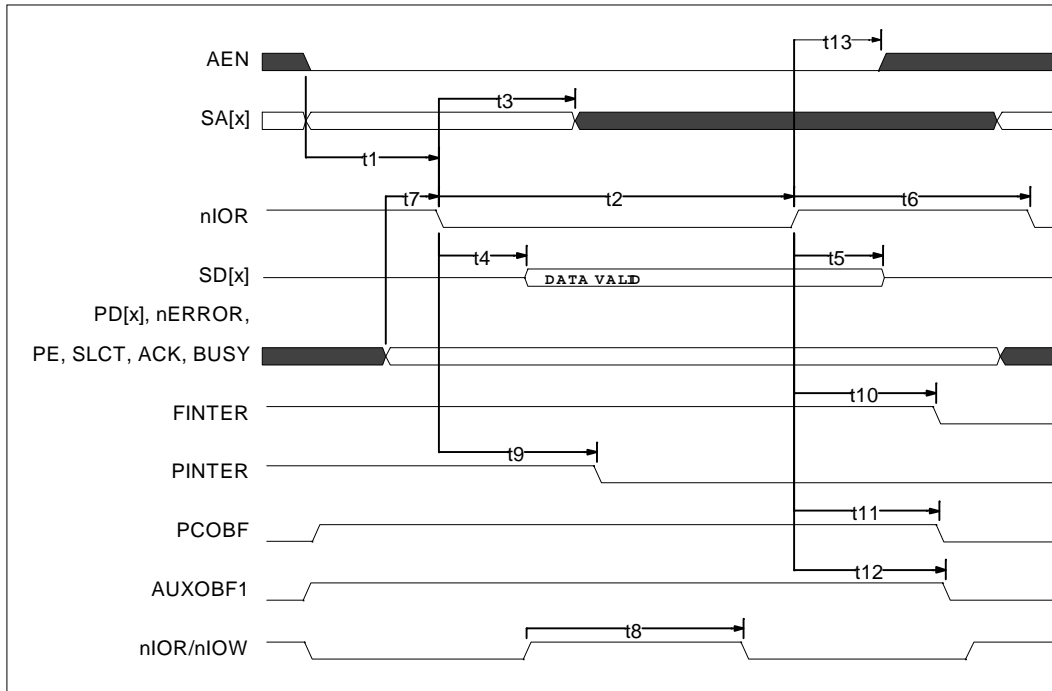
FIGURE 32 - ISA IO READ CYCLE
