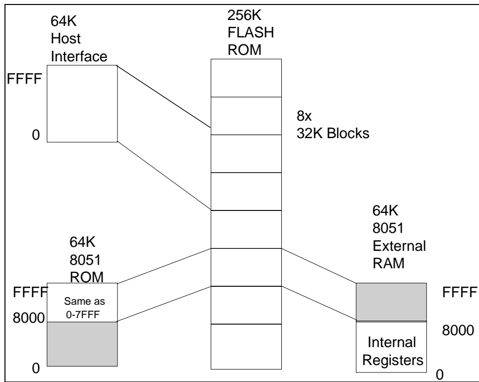
FIGURE 10 - 8051 MODE 2
