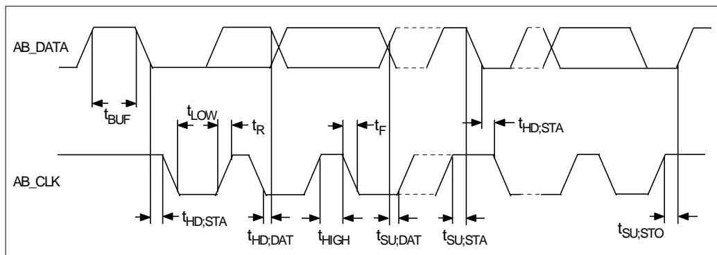
FIGURE 46 - ACCESS.bus TIMING
