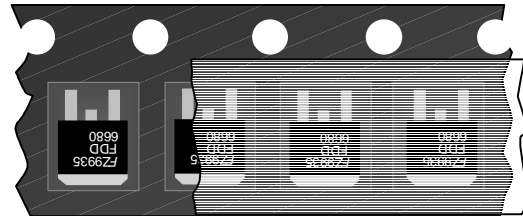
D-PAK (TO-252) Unit Orientation
