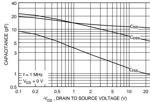
Figure 18. Capacitance Characteristics.
