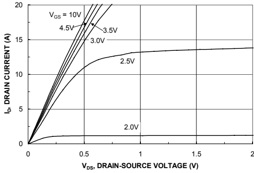
Figure 1. On-Region haracteristics.
