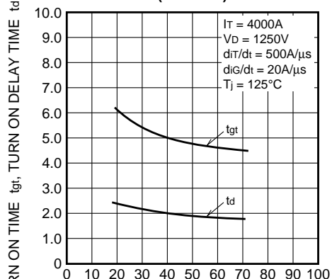
TURN ON GATE CURRENT (A)
