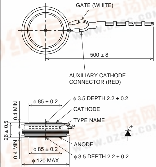
OUTLINE DRAWING
