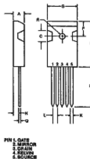
TO-247 (5 LEADED)
