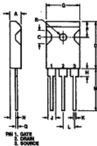
TO-247 (3 LEADED)
