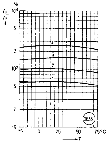
Current transfer ratio (typ.) versus temperature ( I_F = 10 \text{ mA} , V_{CE} = 6 \text{ V} )
