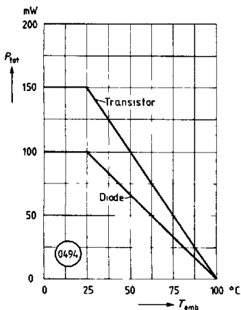
Permissible power dissipation versus ambient temperature
