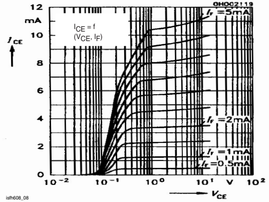
Figure 8. Output Characteristics
