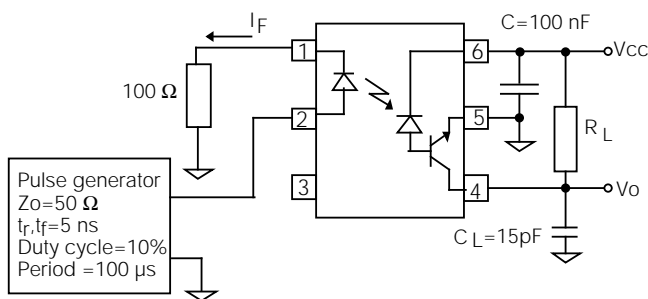
Figure 1. Test set-up
