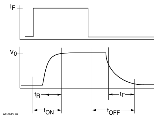
Fig. 2 Switching Waveform
