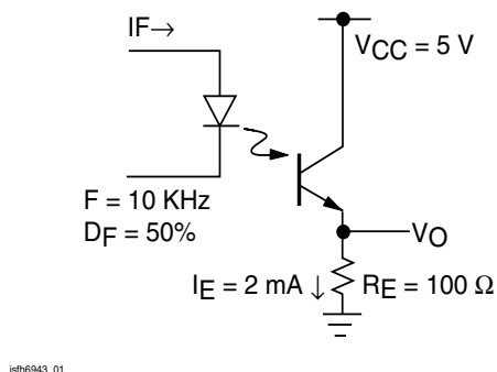
Fig. 1 Switching times (typ.)
