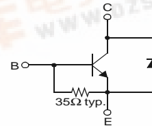
TO-3PF 1.Base 2.Collector 3.Emitter
