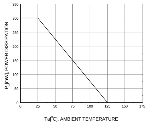
Figure 4. Power Derating
