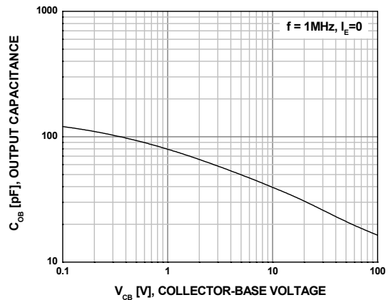
Figure 6. Output Capacitance
