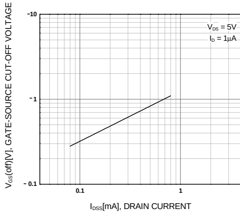
Figure 5. V_{GS(off)} - I_{DSS}
