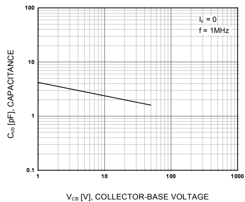
Figure 6. Output Capacitance
