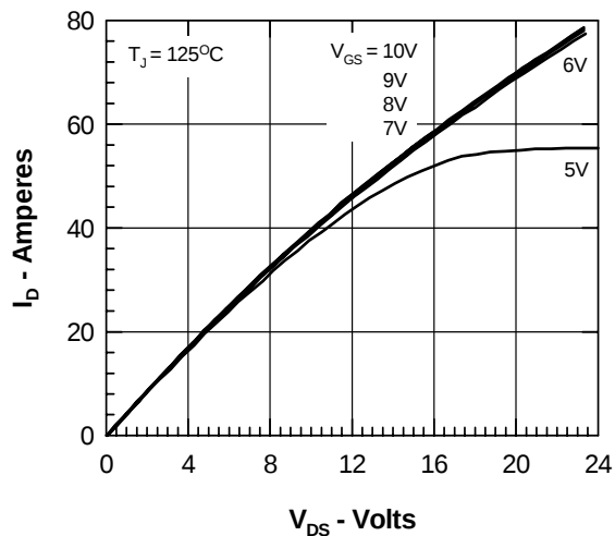
Figure 2. Output Characteristics at 125°C
