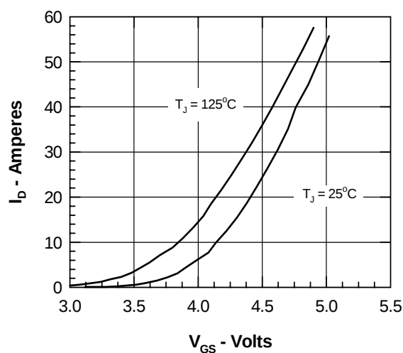
Figure 6. Admittance Curves
