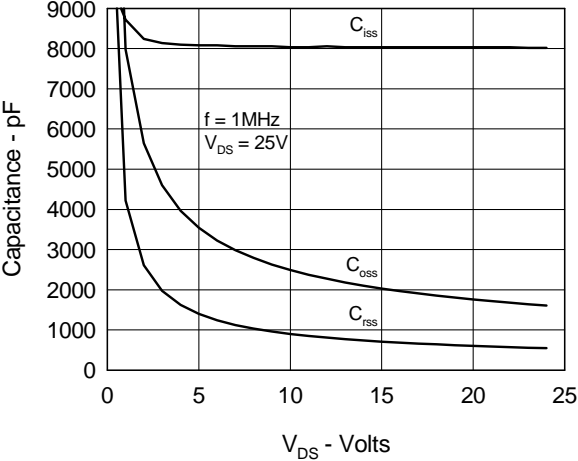
Fig.8 Capacitance Curves
