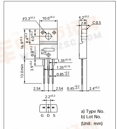
External Dimensions FM20 (full-mold)
