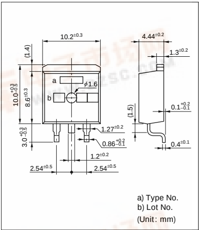
External Dimensions TO220S
