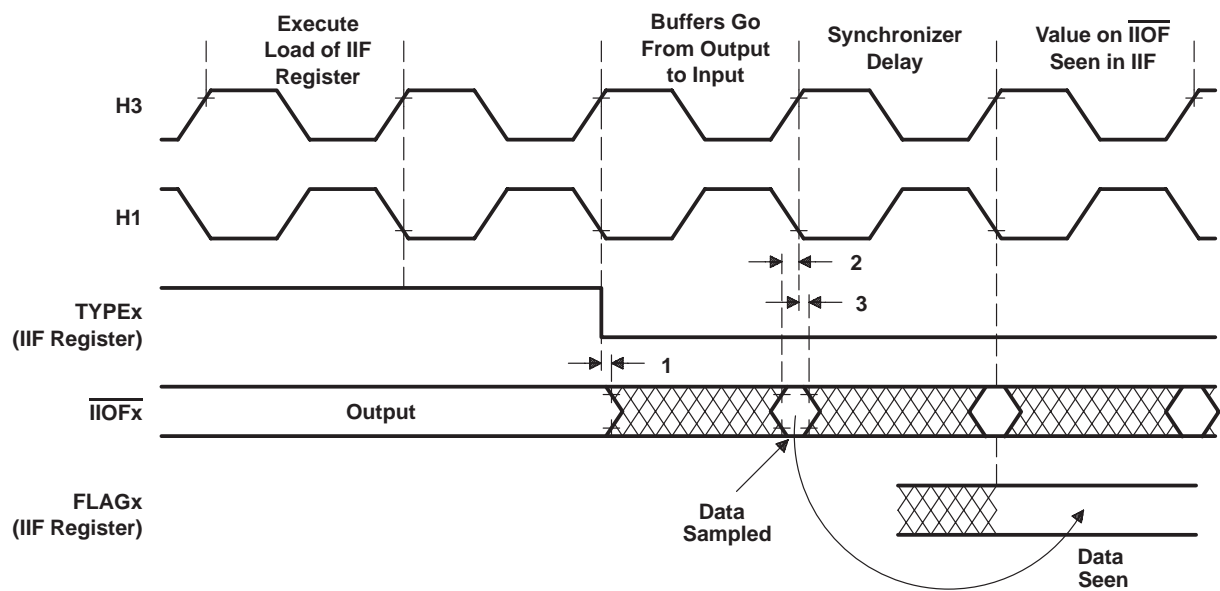
Figure 17. Change of \overline{\text{IIOF}}_x From Output to Input Mode
