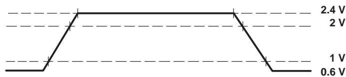
Figure 5. TTL-Level Outputs
