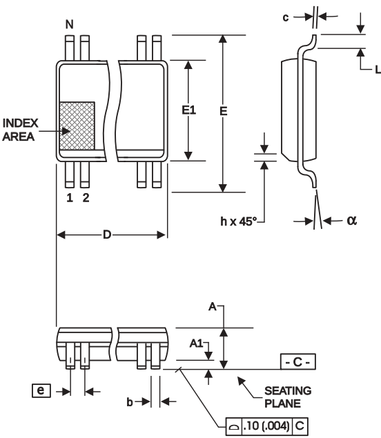
300 mil SSOP Package
