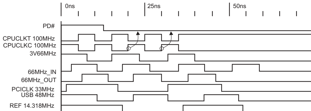
Power Down Assertion of Waveforms
