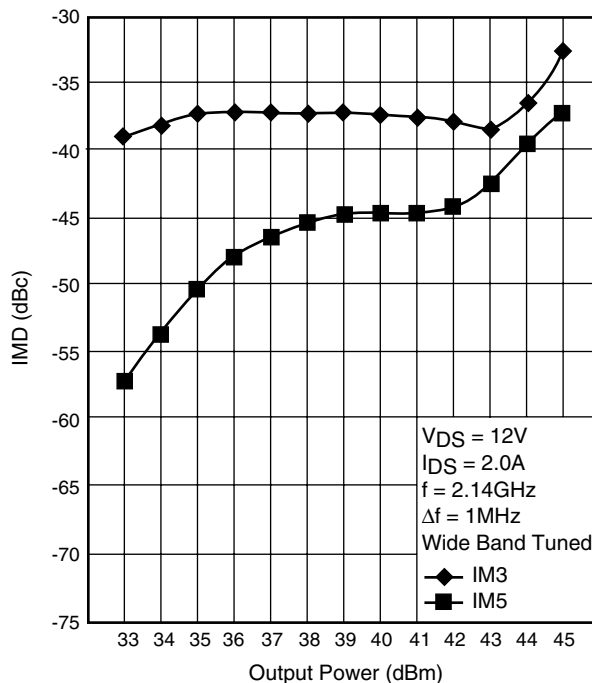
IMD vs. OUTPUT POWER
