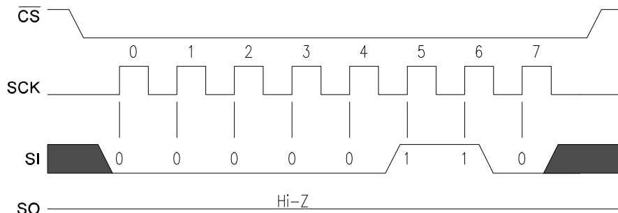
Figure 4. WREN Bus Configuration
