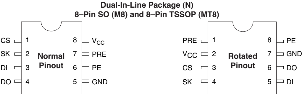
Top View Package Number N08E, M08A and MTC08
