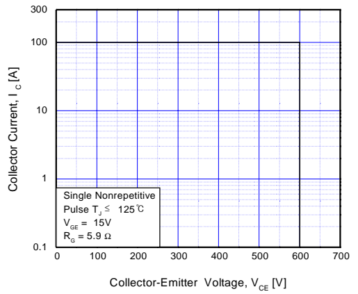
Fig 17. RBSOA Characteristics
