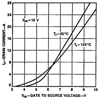
Figure 3 Transfer Characteristics
