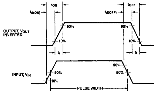
Figure 10 Switching Waveforms
