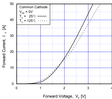
Figure 17. Forward Characteristics
