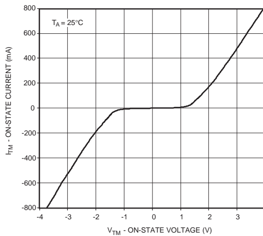
Fig. 7 On-State Characteristics
