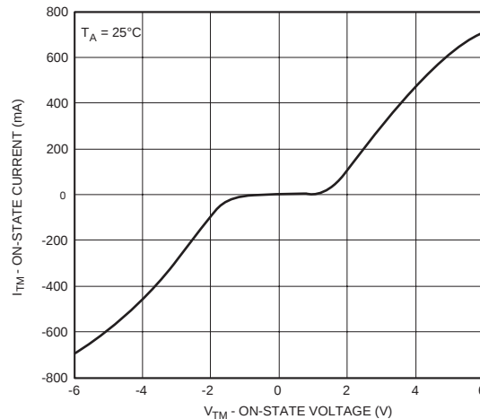
Fig. 7 On-State Characteristics
