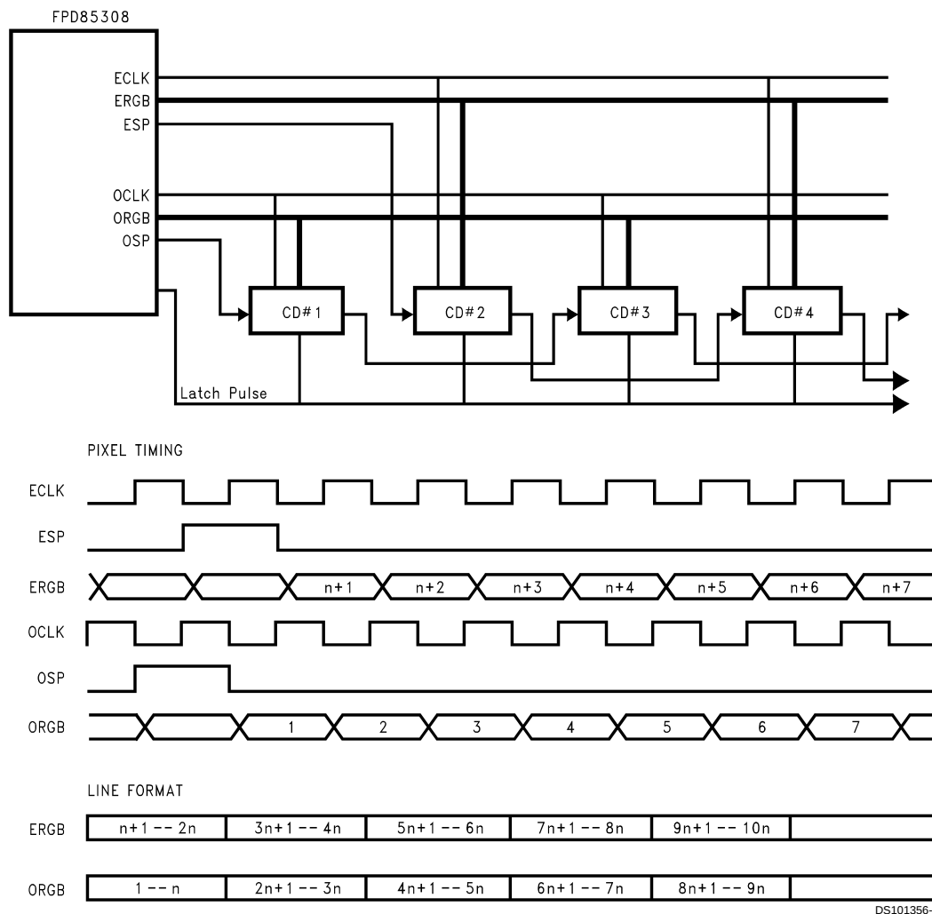
FIGURE 13. Dual Bus Single Port Column Driver Interface (Skewed outputs)
