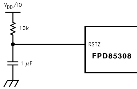
FIGURE 19. Delay Circuit for Stable RSTZ
