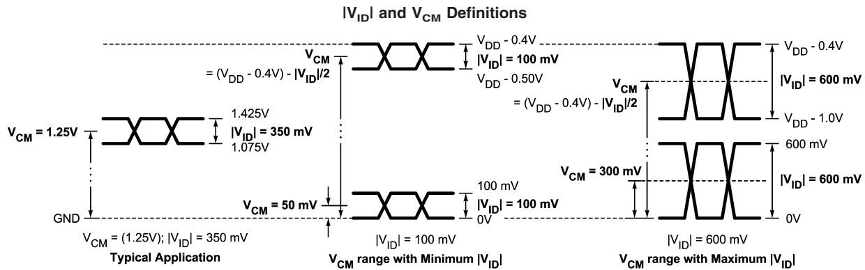
FIGURE 2. LVDS V_{ID} and V_{CM} Allowable Operating Range
