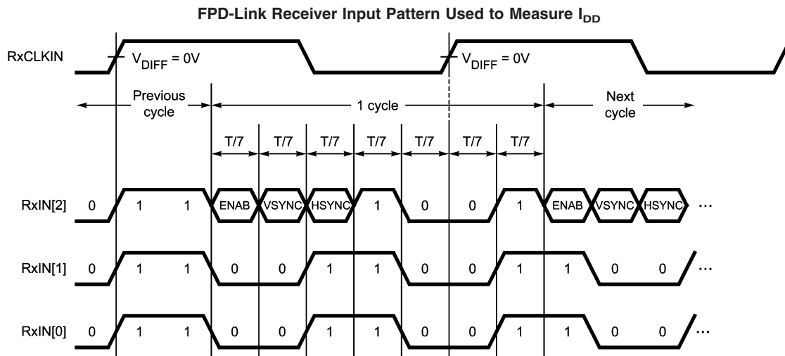
FIGURE 3. FPD-Link Receiver I_{DD} Pattern
