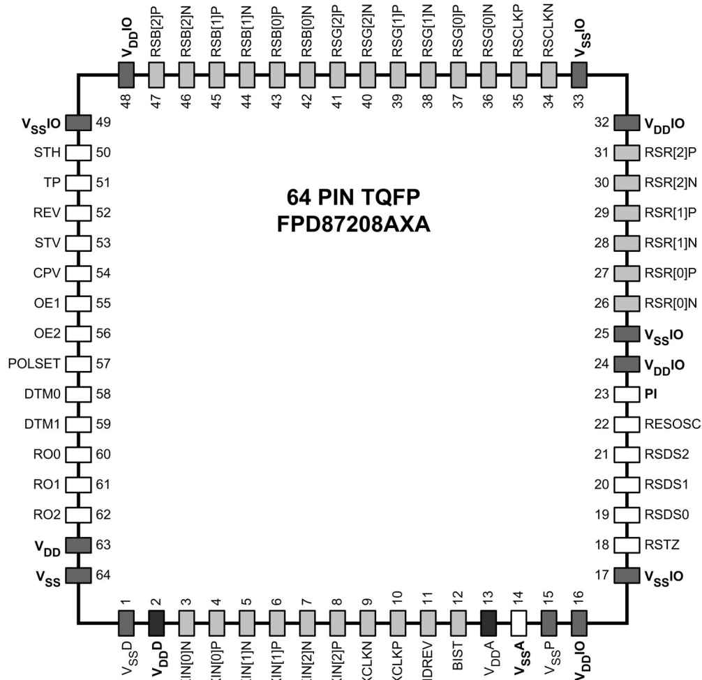
FIGURE 16. Pinout Assignment
