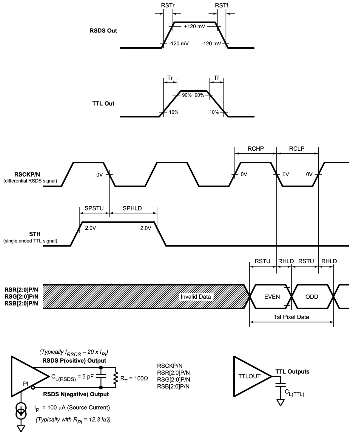
FIGURE 11. RS and TTL Output Timing Diagram
