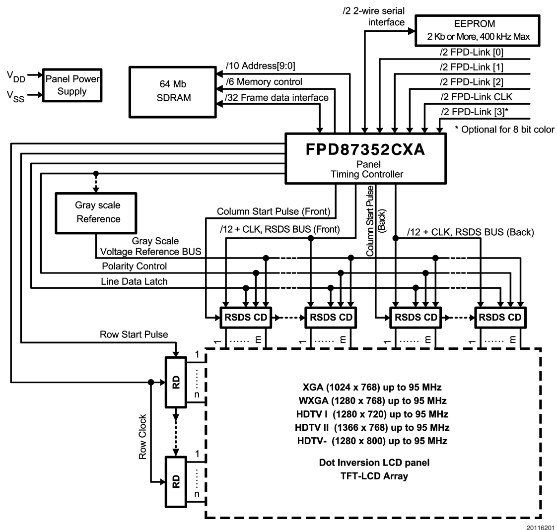
FIGURE 1. Block Diagram of the LCD Module
