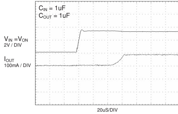
Figure 20. Current-Limit Response
