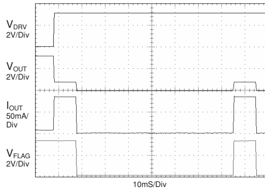
Figure 12. Auto-Restart Time Response
