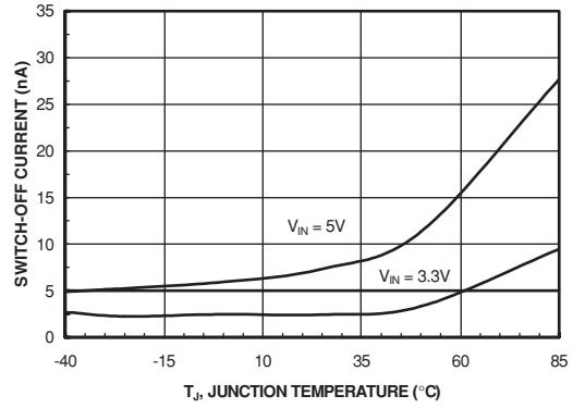
Figure 8. Switch-Off Current vs. Temperature
