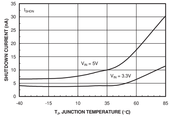
Figure 4. Shutdown Supply Current vs. Temperature
