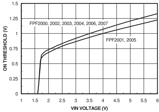
Figure 9. ON Threshold vs. V_{IN}
