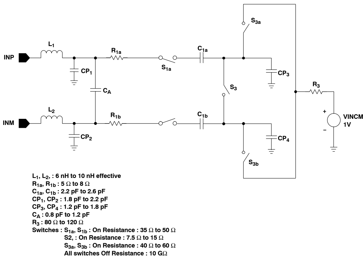
Figure 28. Analog Input Stage
