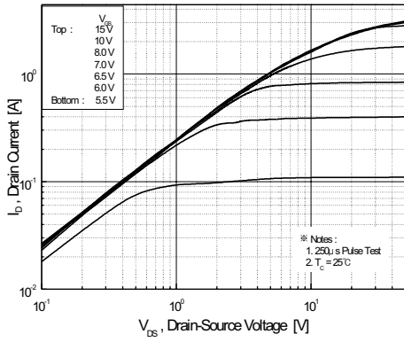
Figure 1. On-Region Characteristics
