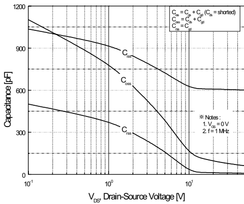
Figure 5. Capacitance Characteristic.
