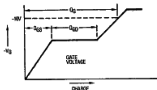
Fig. 16a — Basic Gate Charge Waveform
