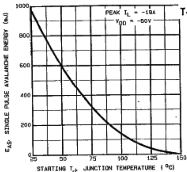
Fig. 14c — Maximum Avalanche Vs. Starting Junction Temperature
