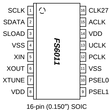
Figure 2: Pin Configuration
