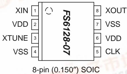
Figure 1: Pin Configuration
