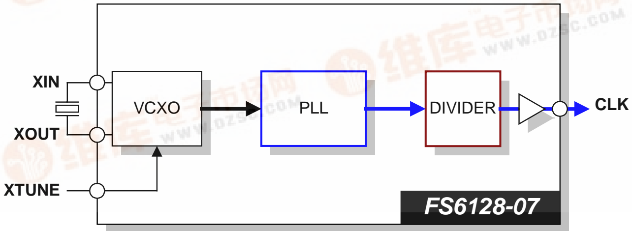
Figure 2: Block Diagram
