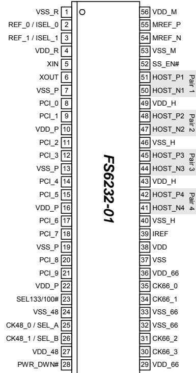
Figure 2: Pin Configuration
