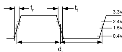
Figure 6: AC Measurement Diagram
