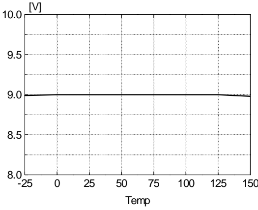
Figure 4. Stop Threshold Voltage vs. Temp
