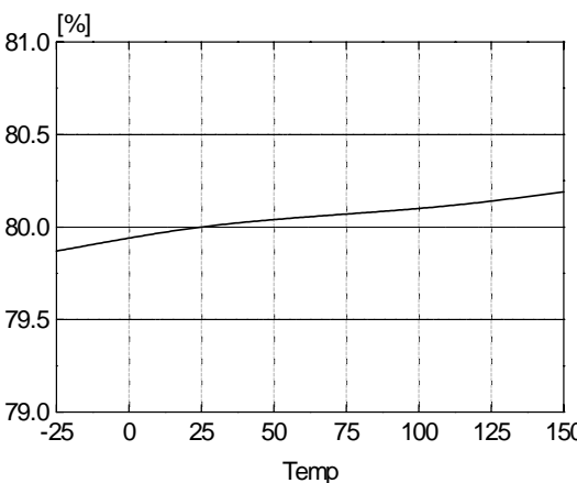
Figure 6. Maximum Duty vs. Temp
