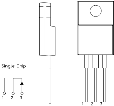
OULINE DRAWING
